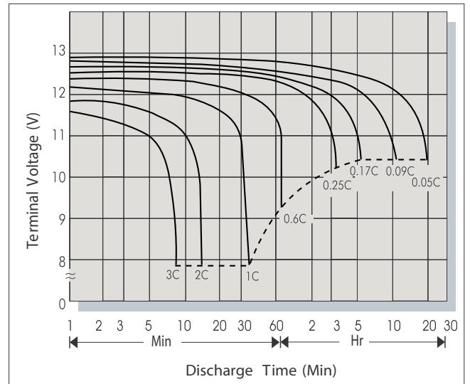
Discharge Current VS. Discharge Voltage
