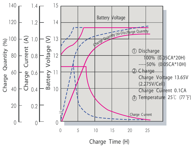
Battery Voltage and Charge Time for Cycle Use
